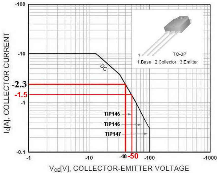
Figure 5. Safe Operating Area
