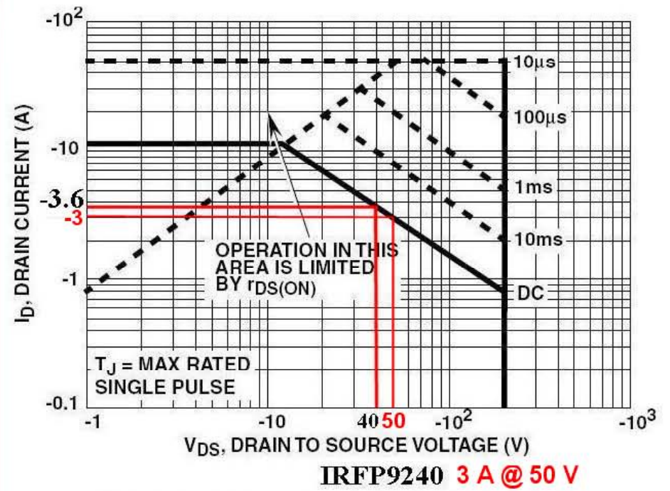
FIGURE 4. FORWARD BIAS SAFE OPERATING AREA
